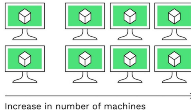
Horizontal scaling
